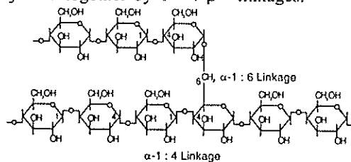
Structure of starch
