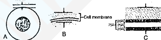
The cell membrane : (A) Light microscope view. (B) and (C) Electron microscope views.
